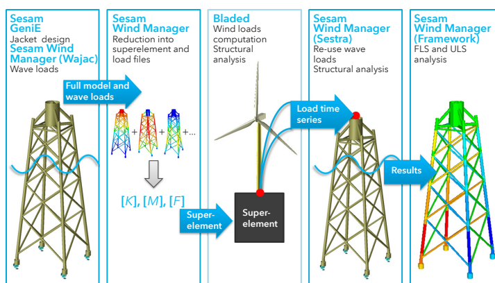
Superelement analysis workflow when using Sesam and Bladed
