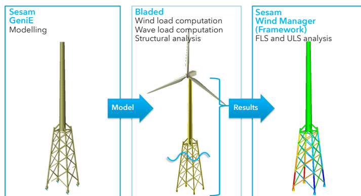
Integrated analysis workflow when using Sesam and Bladed
